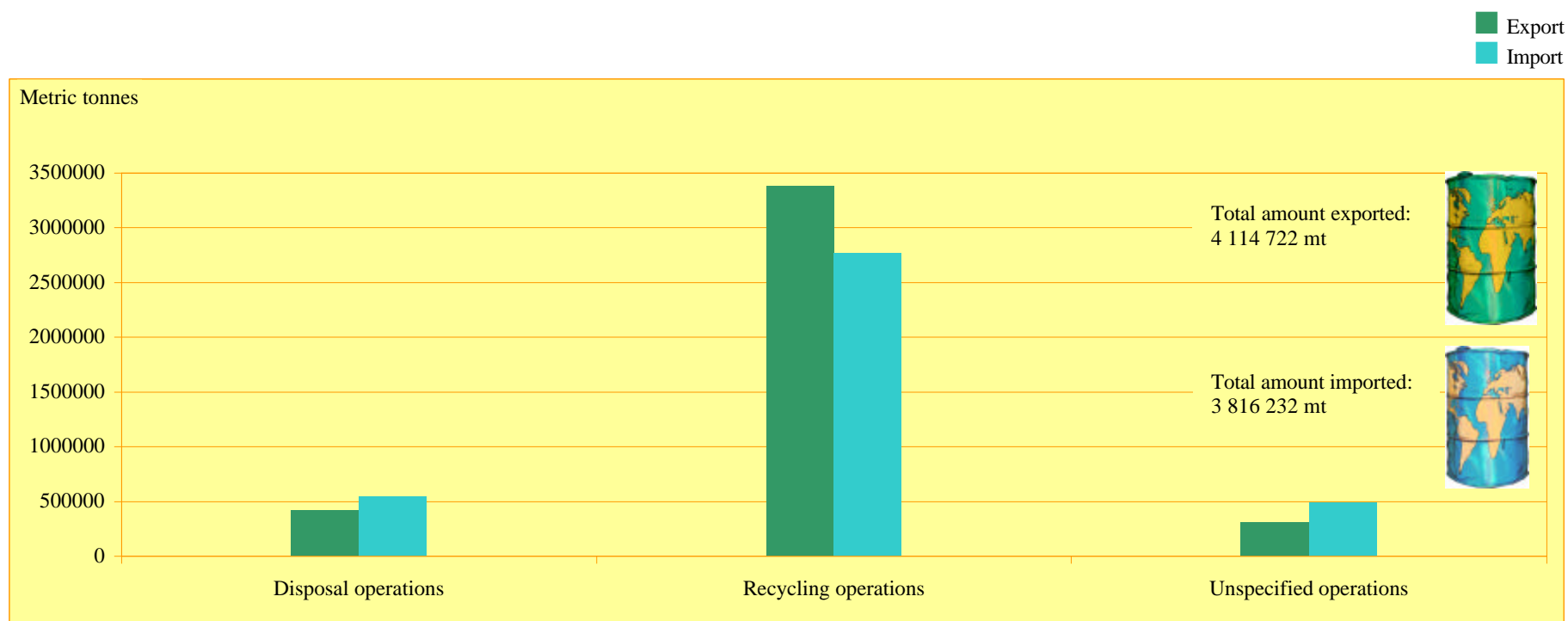
Figure 7: Transboundary Movement of Hazardous Wastes and Other Wastes by Operation among all reporting Parties in 1998
