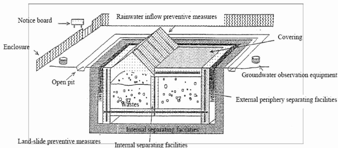
Figure -6 Specially engineered landfill (Ministry of the Environment, Japan 2007a)
