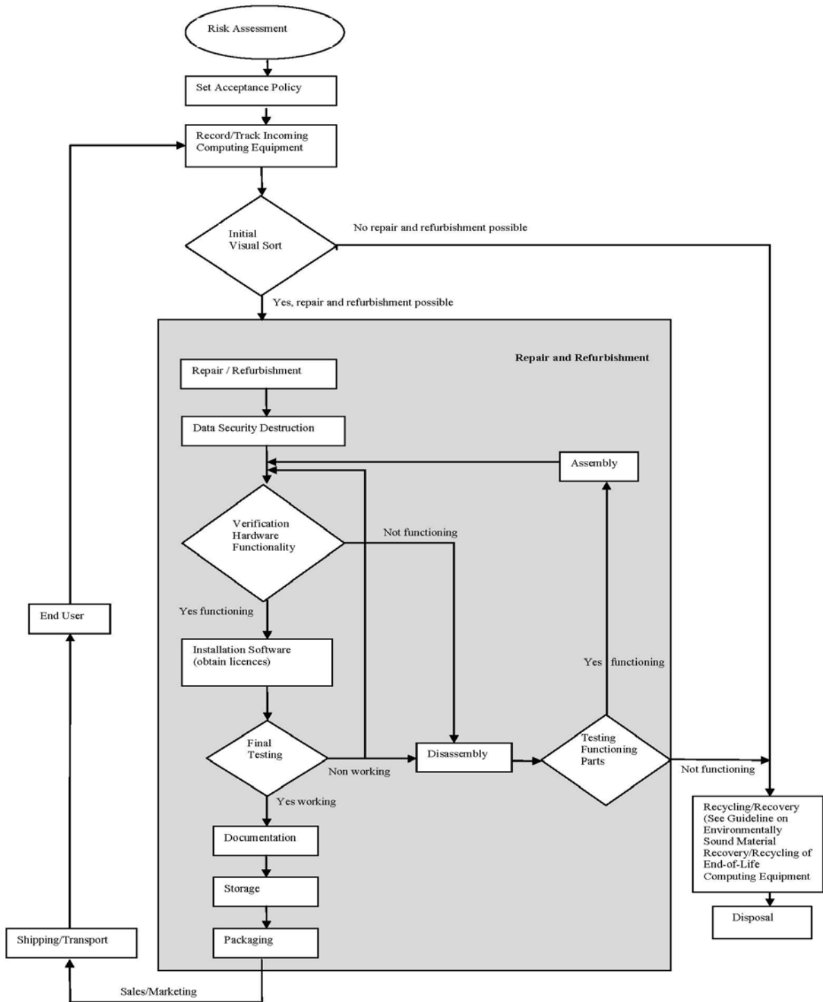
Figure 2 below is an example flow chart showing the environmentally sound refurbishment and repair process in a typical facility
