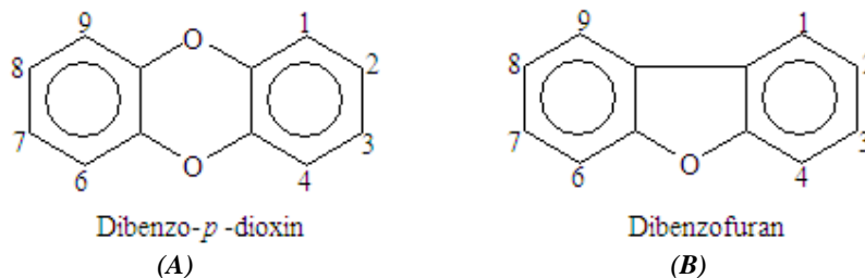
Figure 1: Structures of dibenzo- para -dioxin (A) and dibenzofuran (B)
