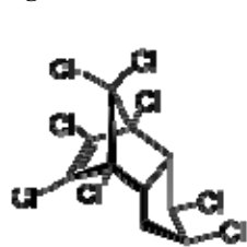
cis-chlordane (also known as \alpha -chlordane)
