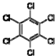
Figure 7: Structure of hexachlorobenzene
