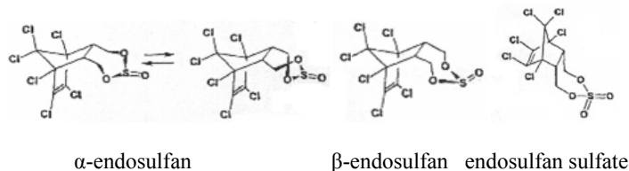
Figure 12: Structure of endosulfan isomers
