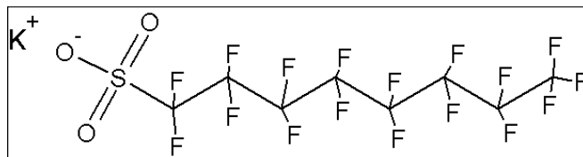
Figure 11: Structure of PFOS
