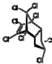
trans-chlordane (also known as \gamma -chlordane)
