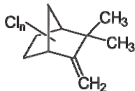
Figure 13: Structure of toxaphene
