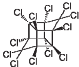
Figure 9: Structure of mirex
