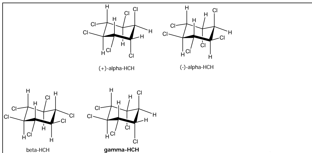
Figure 8: Structure of hexachlorocyclohexane POPs isomers
