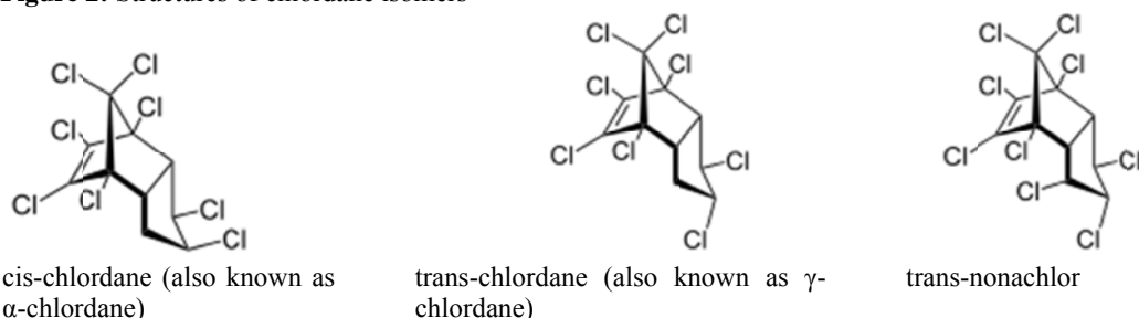
Figure 2: Structures of chlordane isomers
